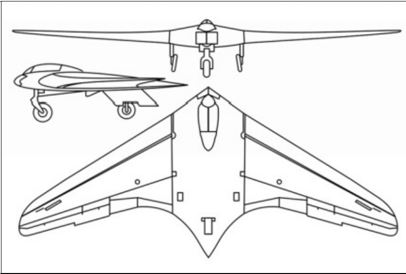
Figure 6. Horton HO-229
